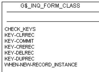
Figure 4: Subclass G$_INQ_FORM_CLASS
