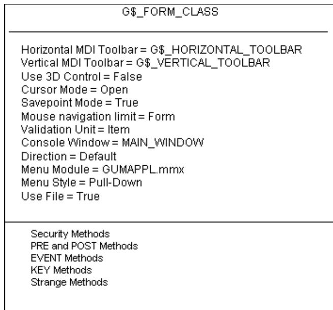
Figure 1: Superclass G$_FORM_CLASS
