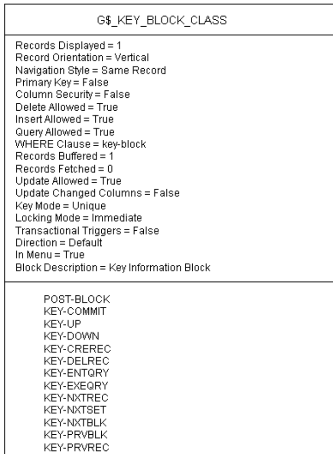
Figure 8: Key Block class
