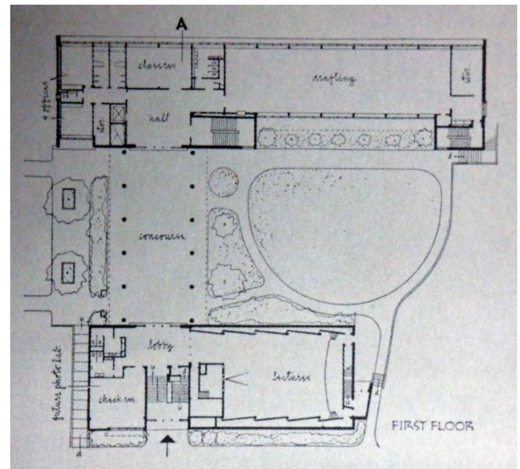
Architecture Bldg, Georgia Tech, 1952 [P. M. Heffernan] [right, top & bot]
